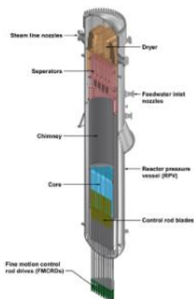
Reactor Pressure Vessel
